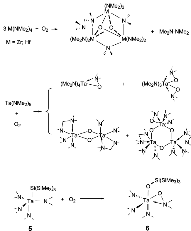
Scheme 1. Reactions of M(\text{NMe}_2)_n ( n = 4 , M = \text{Zr, Hf} ; n = 5 , M = \text{Ta} ) and 5 with \text{O}_2 19–21
