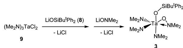
Scheme 5. Preparation of 3 from the Reaction of 9 with 8 and LiONMe 2
