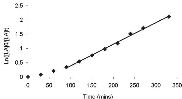
Figure 10. First order plot for rac -LA consumption using \text{Zr}(\text{L}^{\text{OMe}})(\text{O}^i\text{Pr})_2 ( 15 ). Conditions [\text{rac-LA}]_0/[\textbf{15}] = 100:1 , 6 mL of toluene, 70^\circ\text{C} , 0.1 mL aliquots taken at the given intervals. See Experimental Section for other details. Linear fit ( r^2 = 0.996 ) shown is for the first order region after the induction period.
