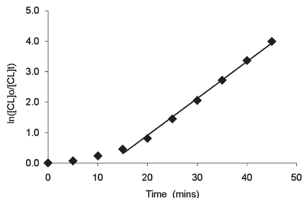
Figure 7. First order plot for \epsilon -CL consumption using \text{Zr}(\text{L}^{\text{OMe}})(\text{O}^i\text{Pr})_2 ( 15 ). Conditions: [\epsilon\text{-CL}_0]/[\textbf{15}] = 100:1 , 6.8 mL of toluene, 100 °C, 0.1 mL aliquots taken at the given intervals. See Experimental Section for other details. Linear fit ( r^2 = 0.995 ) shown is for the first order region after the induction period. See the Supporting Information for corresponding plots for 12 , 13 , and 14 .
