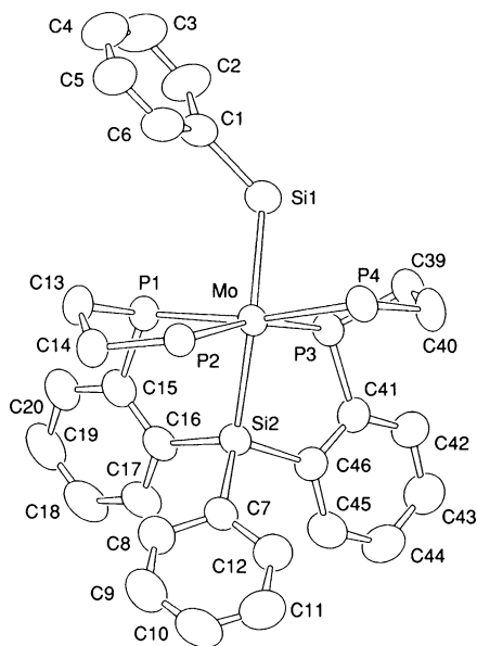
Figure 2. ORTEP drawing of the molecular structure of 4 .
