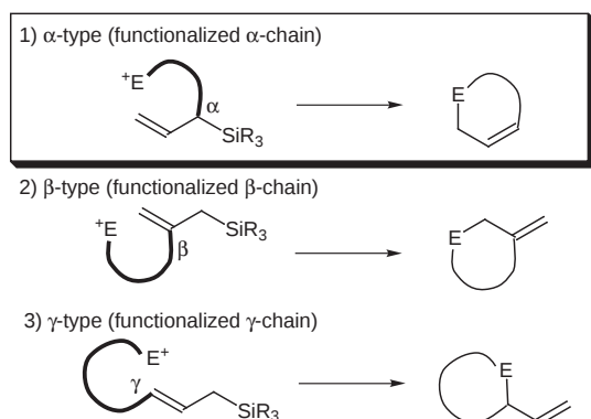
Scheme 1 Classification of Lewis Acid-Promoted Allylsilane Cyclization
