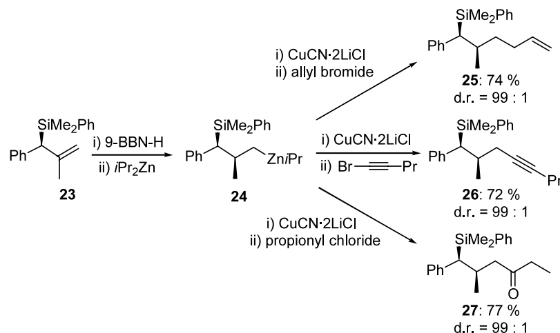
Scheme 7.
