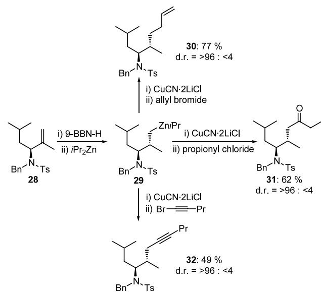
Scheme 8.
