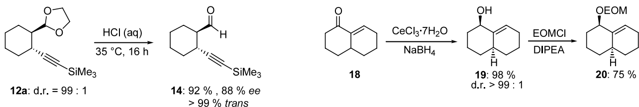
Scheme 4.
