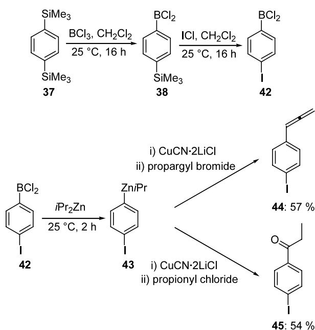
Scheme 11.
