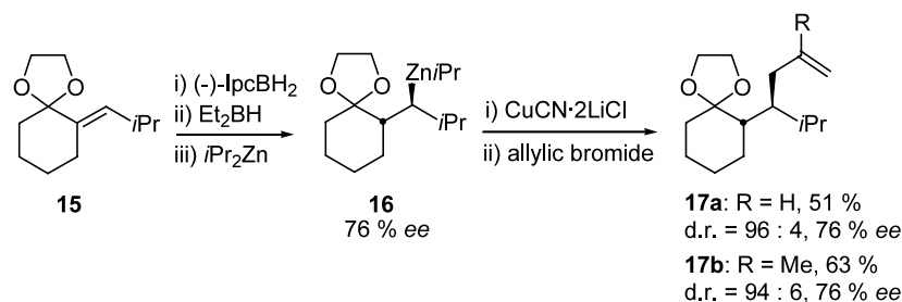
Scheme 5.
