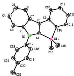
Figure 1. ORTEP drawing of 3a with 30% thermal ellipsoids. Hydrogen atoms have been omitted for clarity.
