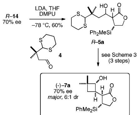
Scheme 9. Cyclization of an Enantiomerically Enriched Substrate
