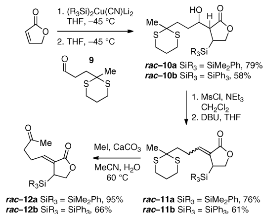
Scheme 5. Four-Step Synthesis of Cyclization Substrates
