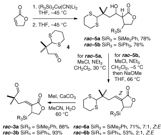
Scheme 3. Three-Step Synthesis of Cyclization Substrates
