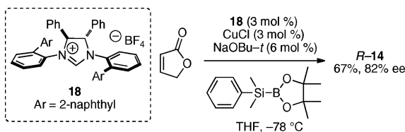
Scheme 8. Improved Asymmetric Approach to Cyclization Substrates
