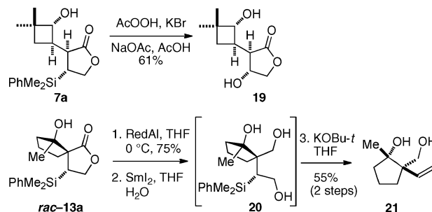
Scheme 10. Manipulation of the C–Si Bond in Cyclization Products
