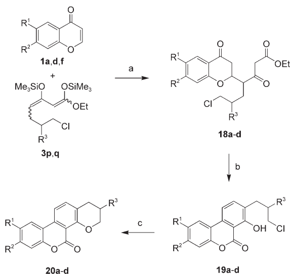
Scheme 8. Synthesis of 2,3-dihydro-1 H -4,6-dioxachrysen-5-ones 20a-d : a) 1) Me 3 SiOTf (1.3 equiv), 0°C, 1 h; 2) 3p,q (1.3 equiv), CH 2 Cl 2 , 12 h; 3) HCl (10%); b) NEt 3 , EtOH, 12 h, 20°C; c) NaH (1.5 equiv), TBAI (2.0 equiv), THF, 20°C, 20 h.
