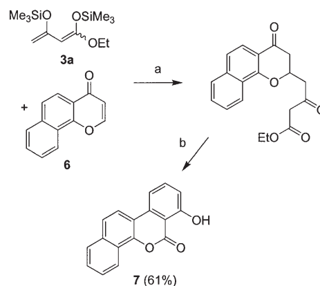
Scheme 5. Synthesis of 7-hydroxydibenzo[ c,d ]chromen-6-one 7 : a) 1) Me 3 SiOTf (1.3 equiv), 20 °C, 1 h; 2) 3a (1.3 equiv), CH 2 Cl 2 , 0 → 20 °C, 12 h; 3) HCl (10%); b) NEt 3 (2.0 equiv), EtOH, 20 °C, 12 h.
