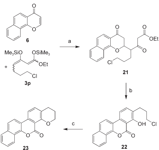
Scheme 9. Synthesis of 3,4-dihydro-2 H -1,13-dioxapicen-14-one 23 : a) 1) Me 3 SiOTf (1.3 equiv), 0°C, 1 h; 2) 3p (1.3 equiv), CH 2 Cl 2 , 12 h; 3) HCl (10%); b) NEt 3 , EtOH, 12 h, 20°C; c) NaH (1.5 equiv), TBAI (2.0 equiv), THF, 20°C, 20 h.
