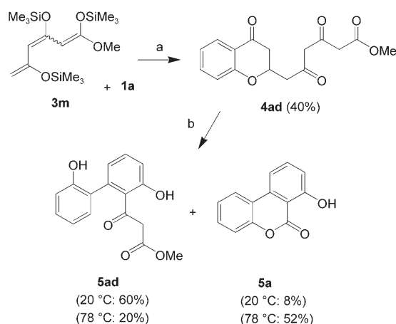
Scheme 2. Reaction of 1,3,5-trisilyl enol ether 3m with 1a : a) 1) Me 3 SiOTf (1.3 equiv), 20 °C, 1 h; 2) 3m (1.3 equiv), CH 2 Cl 2 , 0 → 20 °C, 12 h; 3) HCl (10%); b) NEt 3 (2.0 equiv), EtOH (12 h, 20 °C or 3 h, 78 °C).
