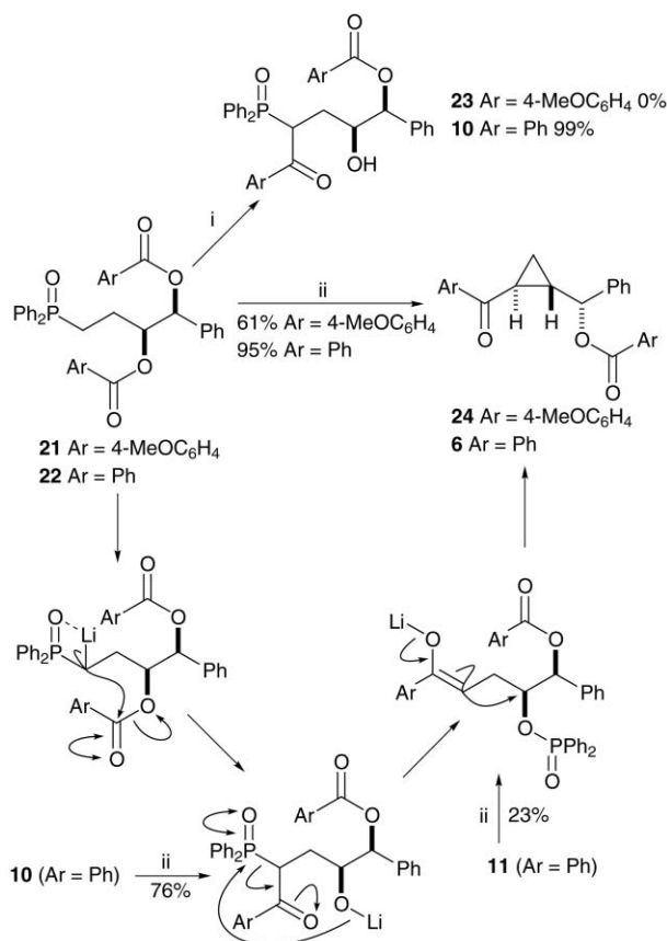
Scheme 7 Reagents and conditions: i, LDA, THF, −78 °C; ii, LDA, THF, −78 °C to 0 °C.
