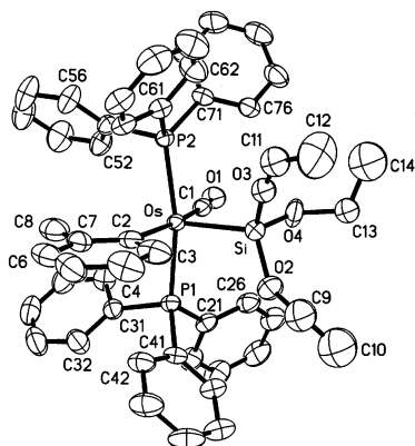
Fig. 3. Molecular geometry of \text{Os}[\text{Si}(\text{OEt})_3](o\text{-tolyl})(\text{CO})(\text{PPh}_3)_2 ( 3b ).
