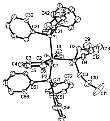
Fig. 2. Molecular geometry of \text{Os}[\text{Si}(\text{OEt})_3](\text{Ph})(\text{CO})(\text{PPh}_3)_2 ( 3a ).
