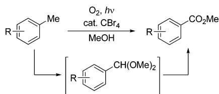
Scheme 1. Direct Synthesis of Methyl Esters via Dimethyl Acetals
