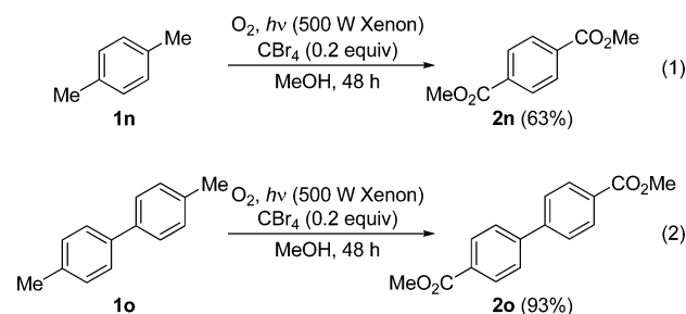
Scheme 2. Direct Aerobic Photo-Oxidative Synthesis of Methyl Esters from Methyl Aromatics
