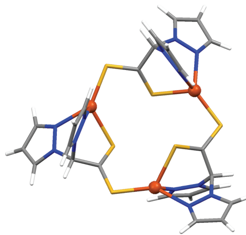
Figure 6. Optimized molecular structure of the [\text{Cu}(\text{L}')_3] complex. 77 Density functional: B3LYP, basis set: Cu, S (lan12dz) C,H,N (6-31G(d)); in \text{L}' , the t\text{-Bu} of \text{L} are replaced by H atoms to save computational resources). Selected bond distances: Cu–N, 2.16–2.22 Å range; Cu–S bridge , 2.31–2.32 Å range; Cu–S chelate , 2.47–2.51 Å range.
