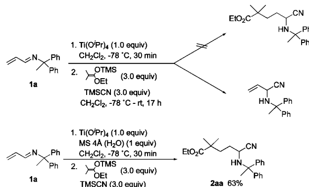
Scheme 2. Double Nucleophilic Additions to N -Allylideneamine
