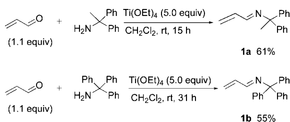
Scheme 1. Preparation of N -Allylideneamines
