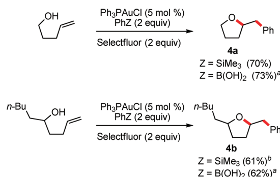
Scheme 2. Two-Component Oxyarylation via Intramolecular Alkoxyacyclization
