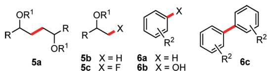
Figure 1. Possible side products of oxyarylation, arising from dimerization 5a , protodeauration 5b , or reductive elimination 5c of an alkylgold fluoride intermediate or protodesilylation 6a or oxidation 6b of arylsilane reagents (not observed). Biaryl 6c , from oxidative homocoupling of the silane reagent, was observed.
