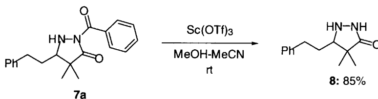
Scheme 7. Removal of Benzoyl Group of 7a
