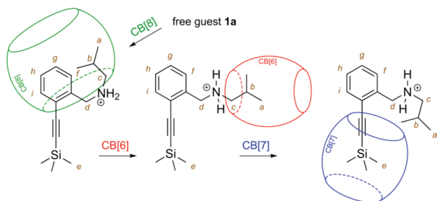
Figure 1. Consecutive site- and host-selective encapsulation of guest 1a with CB[8], CB[6], and CB[7].
