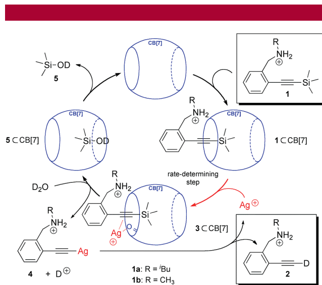
Figure 4. Plausible cycle for CB[ n ]-catalyzed desilylations in the presence of Ag(I) salts in aqueous medium.
