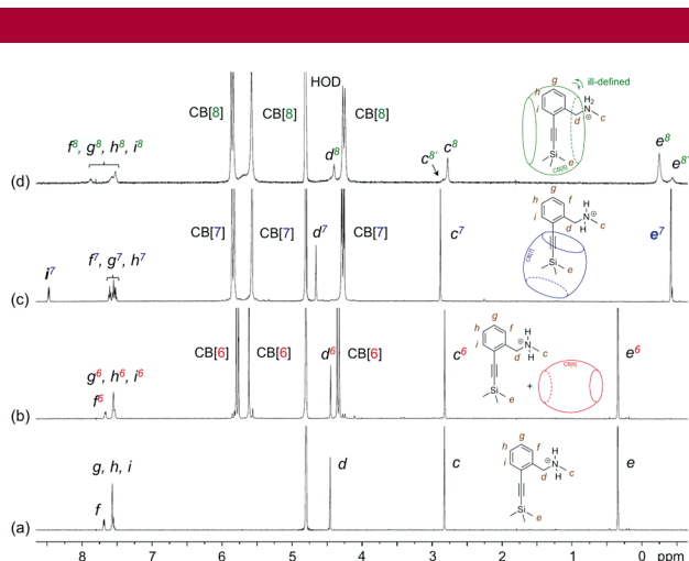
Figure 5. ^1\text{H} NMR spectra of (a) free guest 1b , (b) 1b \subset CB[6], (c) 1b \subset CB[7], and (d) 1b \subset CB[8] (500 MHz; 1.0 mM in \text{D}_2\text{O} , in the presence of 20 mM sodium nitrate).
