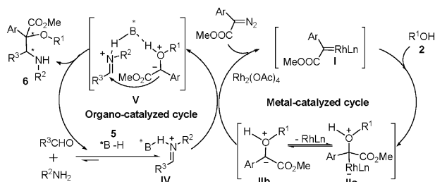
Scheme 3 Proposed mechanism of metal-organocatalytic cooperative catalysis.
