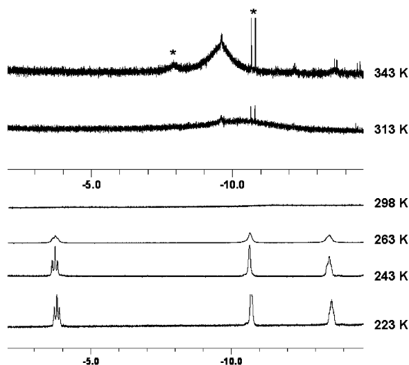
Figure 1. Variable-temperature ^1\text{H} NMR (400 MHz) spectra of 2 in \text{C}_7\text{D}_8 in the hydride region (* indicates impurities).
