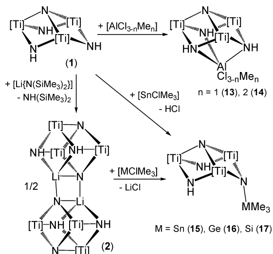
Scheme 3. Reactions with Chloromethyl Complexes [\text{AlCl}_{3-n}\text{Me}_n] and [\text{MClMe}_3] ( [\text{Ti}] = \text{Ti}(\eta^5\text{-C}_5\text{Me}_5) )
