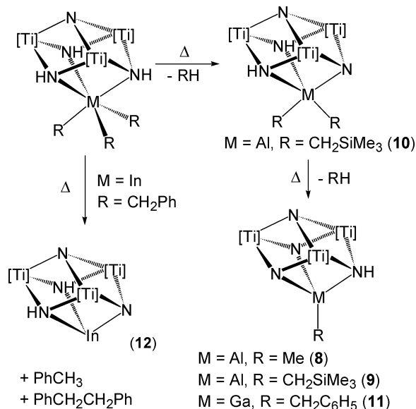
Scheme 2. Thermal Behavior of Adducts [\text{R}_3\text{M}\{(\mu_3\text{-NH})_2\text{Ti}_3(\eta^5\text{-C}_5\text{Me}_5)_3(\mu_3\text{-N})\}] ( [\text{Ti}] = \text{Ti}(\eta^5\text{-C}_5\text{Me}_5) )
