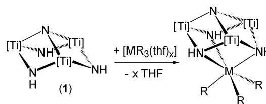
Scheme 1. Reactions of 1 with [\text{MR}_3] ( [\text{Ti}] = \text{Ti}(\eta^5\text{-C}_5\text{Me}_5) )
