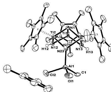
Figure 4. Perspective view of 13 · \text{C}_7\text{H}_8 with thermal ellipsoids at the 50% probability level.
