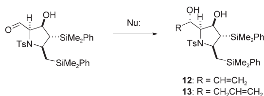
Scheme 4. Allylation/vinylation of 11 .
