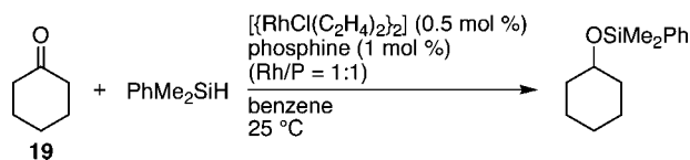
Scheme 2. Rh-Catalyzed Hydrosilylation of Cyclohexanone (19) with PhMe 2 SiH
