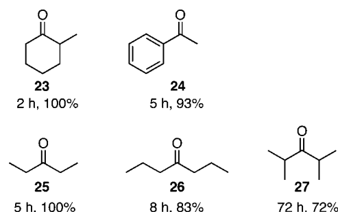
Chart 5. Results (Reaction Time and Conversion) of Hydrosilylation of Various Ketones with PhMe 2 SiH Catalyzed by the Rh-1a System (Rh/P1:1) a
