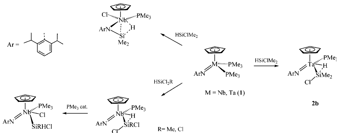
Scheme 1. Reactions of \text{Cp}(\text{ArN})\text{M}(\text{PMe}_3)_2 ( \text{M} = \text{Nb}, \text{Ta} ) with Hydrosilanes
