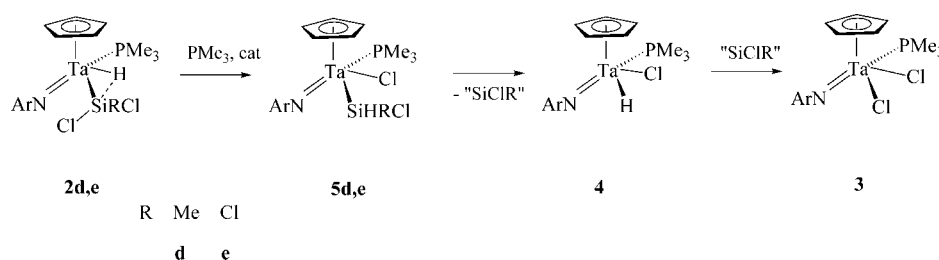
Scheme 2. Decomposition Pathway for Complexes 2d and 2e in Mother Liquor
