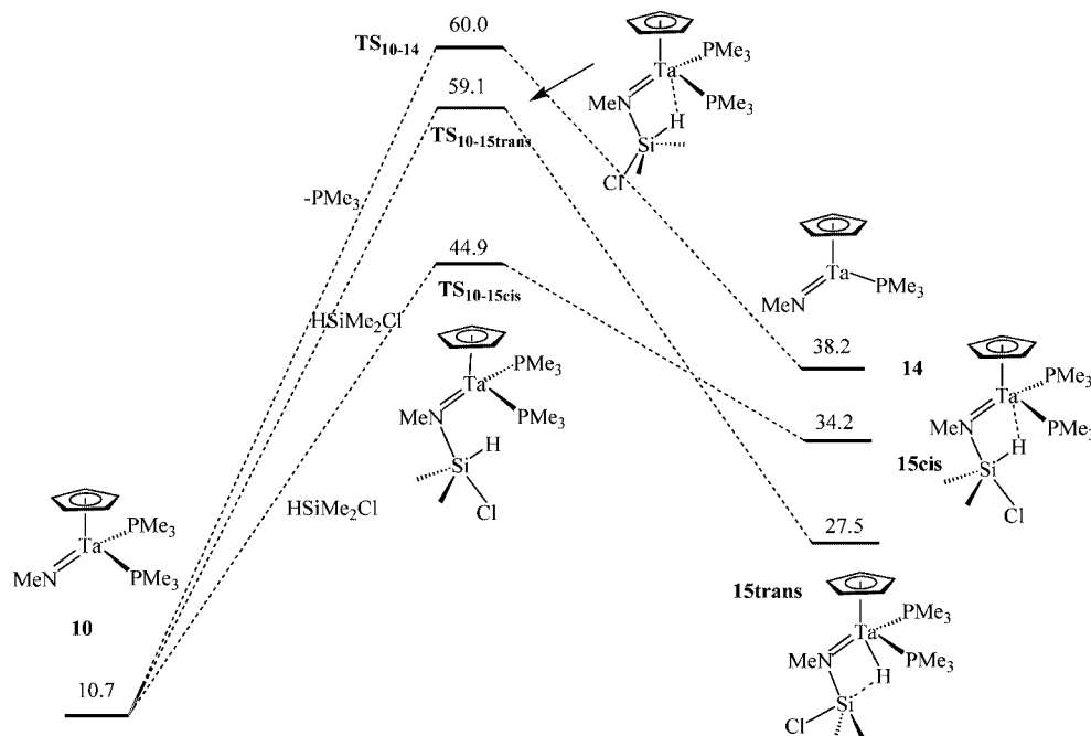
Figure 3. Possible reaction pathways in the reaction between complex 10 and HSiMe 2 Cl. Free energies (in kcal/mol) are taken relative to 11trans .
