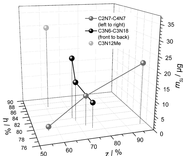
Figure 5. Relationship between the amount of precipitated silica (given as m_{\text{Si}} ), the protonation state z , and the hydrophobic character h of the polyamines C3N6, C3N12, C3N18, C2N7, C3N7, C4N7, and C3N12Me.
