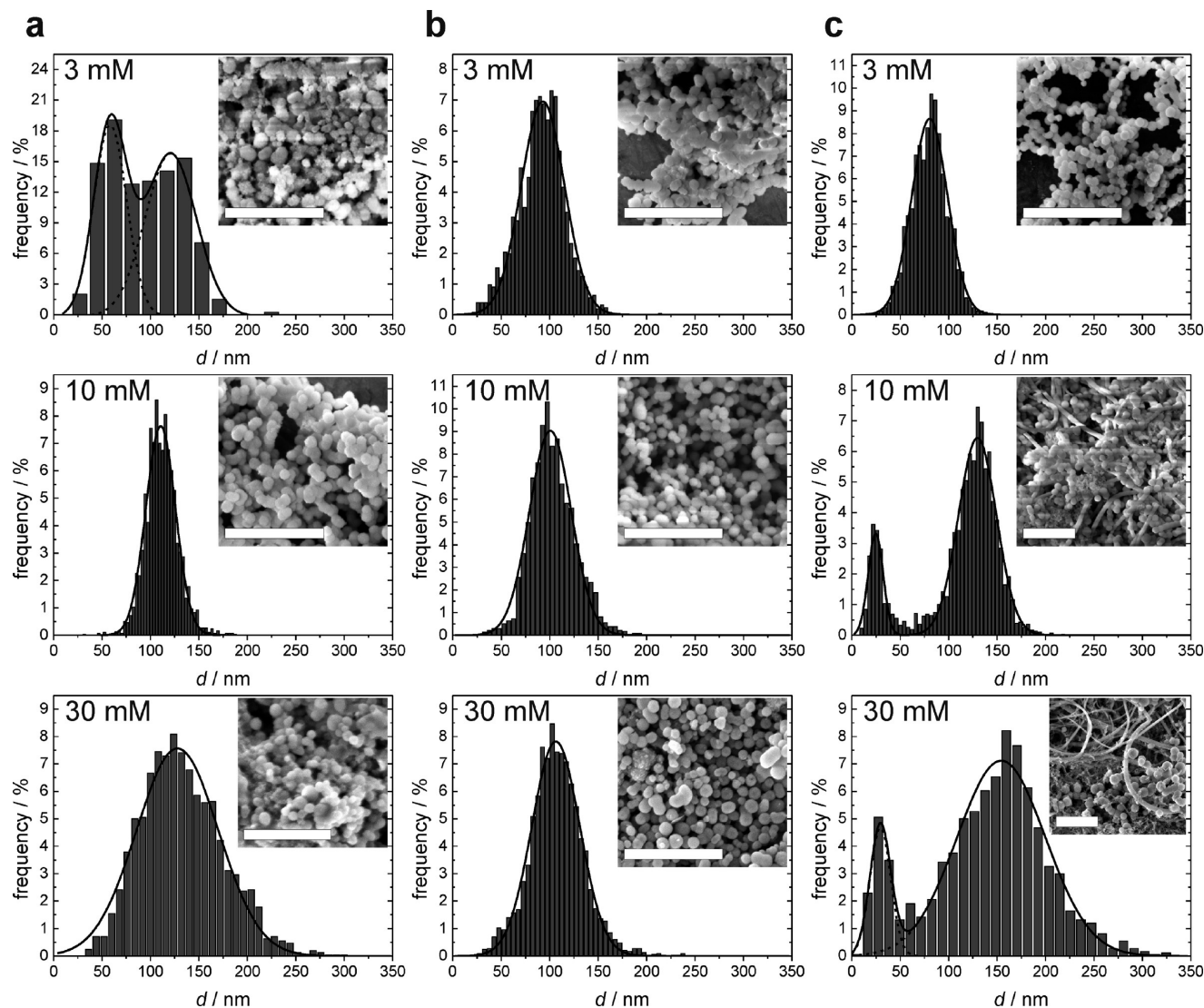
Figure 4. Histogram analyses and corresponding scanning electron micrographs of the silica precipitates obtained in the presence of (a) C3N6, (b) C3N12, and (c) C3N18 using three different phosphate concentrations (3, 10, and 30 mM). Silica precipitates were generated in 30 mM acetate buffer (pH 6.8) with c_N = 1 mM and c_{Si(OH)_4} = 100 mM. Scale bars are 1 \mu m.
