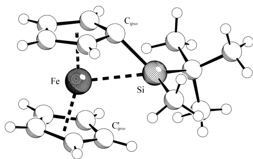
Figure 2. Crystal structure analysis of 3 + : Schakal plot of the molecular structure (counteranion omitted for the sake of clarity). Selected experimental bond lengths (Å): Si–C ipso 1.829(9); Si–Fe, 2.492(2); Si–C' ipso 2.784(9). Selected calculated bond lengths (Å): Si–C ipso 1.823; Si–Fe, 2.461; Si–C' ipso 2.647.
