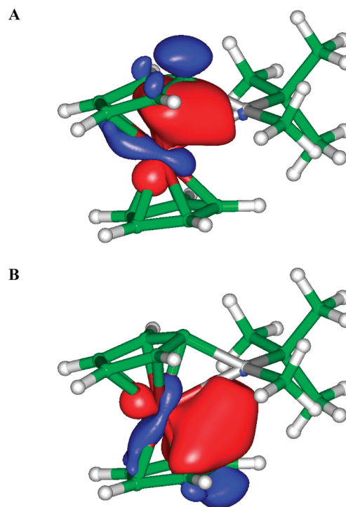
Figure 3. Localized molecular orbitals. (A) LMO A and (B) LMO B involving silicon, iron, and ring carbon atoms (isosurfaces are displayed at a value of 0.05 e/a 0 3/2 ). The Mulliken populations of the silicon atomic orbitals in the LMOs are 19.2% for LMO A and 12.5% for LMO B .
