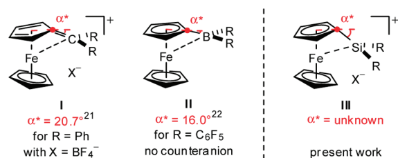
Figure 1. Isoelectronic charged and neutral ferrocene-based systems with an electron sextet at the \alpha atom.
