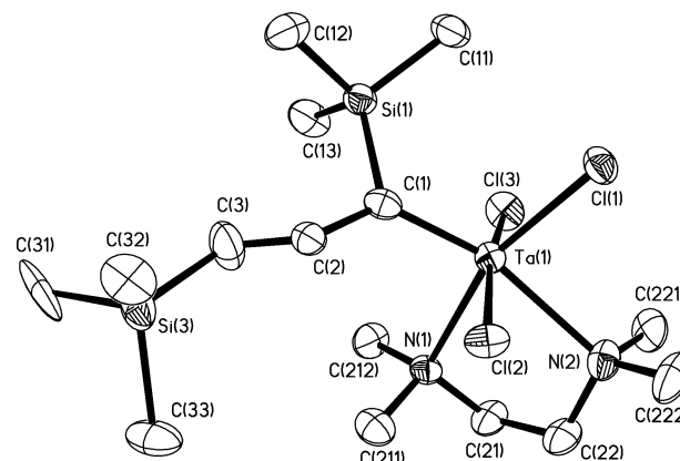
Figure 2. Molecular structure of \text{Me}_3\text{SiCH}=\text{CHC}(\text{SiMe}_3)=\text{TaCl}_3(\text{TMEDA}) ( 5 ). Thermal ellipsoids are drawn at the 50% probability level. Hydrogen atoms are omitted for clarity.
