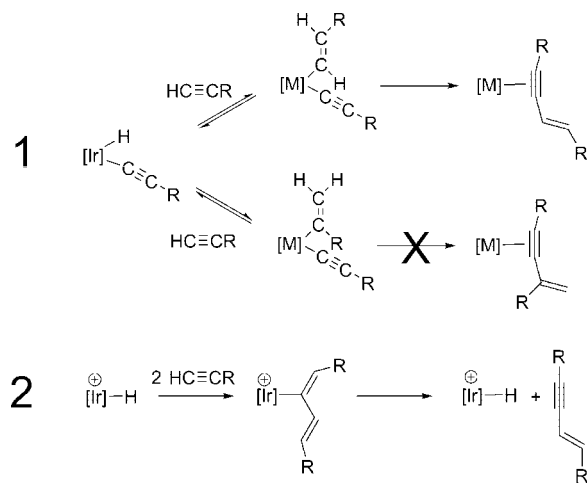
Scheme 1. Alkyne Coupling Pathways Favoring Head-to-Head Coupling Products
