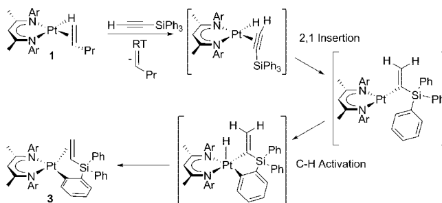
Scheme 2. Formation of 3 via 2,1-Insertion of Ph_3SiC\equiv CH into the Pt–H Bond of 1
