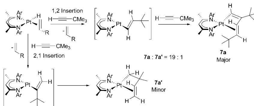
Scheme 4. Two Possible Insertion Pathways for t\text{-BuC}\equiv\text{CH}
