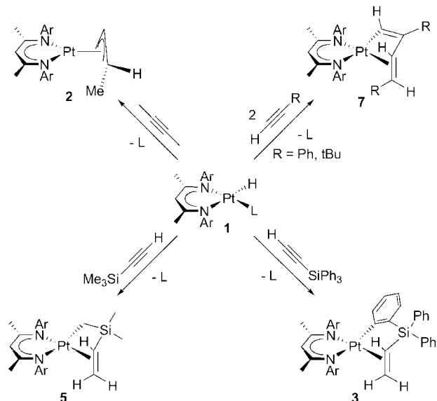
Scheme 6. Addition of Various Alkynes to (Cl-nacnac)Pt(H)(1-pentene) ( 1 )
