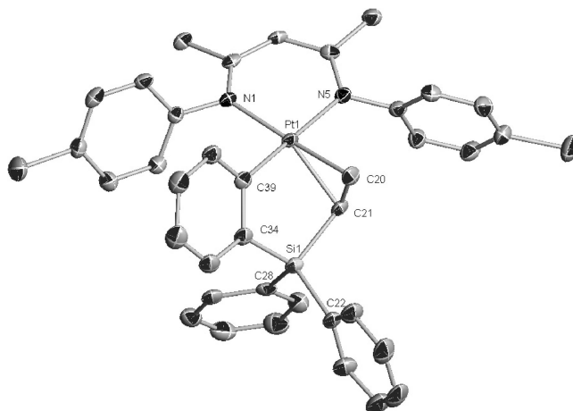
Figure 1. X-ray crystal structure of (Cl\text{-}nacnac)Pt((o\text{-}C_6H_4)Si(Ph)_2(CH=CH_2)) ( 3 ). Selected bond distances ( \text{\AA} ) and angles (deg): Pt1\text{--}C39 = 2.031 ; Pt1\text{--}C20 = 2.142 ; Pt1\text{--}C21 = 2.140 ; Pt1\text{--}N1 = 2.044 ; Pt1\text{--}N5 = 2.120 ; C20\text{--}C21 = 1.404 ; C39\text{--}Pt1\text{--}C20 = 82.62 ; C39\text{--}Pt1\text{--}C21 = 86.12 ; C34\text{--}Si1\text{--}C21 = 100.2 ; N1\text{--}Pt1\text{--}C20 = 150.97 ; N1\text{--}Pt1\text{--}C21 = 169.33 ; N1\text{--}Pt1\text{--}N5 = 91.02 .
