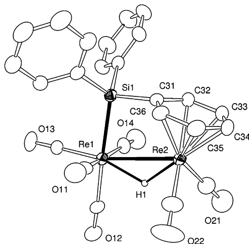
Figure 2. ORTEP diagram of the molecular structure of Re 2 (CO) 6 ( \eta^7 -SiPh 3 )( \mu -H) ( 6 ) showing 40% thermal ellipsoid probability. Selected intramolecular distances (Å) and angles (deg): Re(1)–Re(2) = 3.2192(2), Re(1)–Si(1) = 2.5175(11), Si(1)–C(31) = 1.905(4), Re(1)–H(1) = 1.894(10), Re(2)–H(1) = 1.897(10), Re(2)–Re(1)–Si(1) = 74.91(2).
