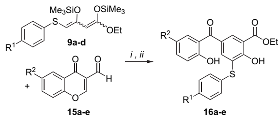
Scheme 5. Synthesis of 16a–e . Reagents and conditions: (i) \text{Me}_3\text{SiOTf} (0.3 equiv), 20^\circ\text{C} , 10 min; (ii) (1): 9a–d (1.3 equiv), \text{CH}_2\text{Cl}_2 , 0 \rightarrow 20^\circ\text{C} , 12 h; (2) HCl (10%).
