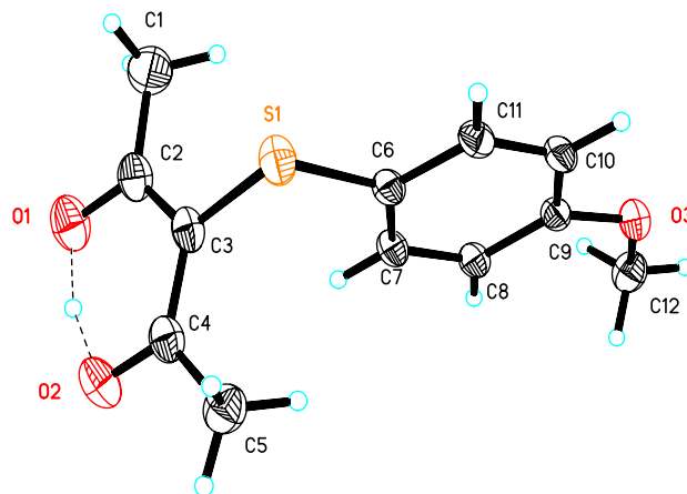
Figure 1. ORTEP plot of 3b (the position of the H atom between O1 and O1 was calculated from the difference map and refined freely).
