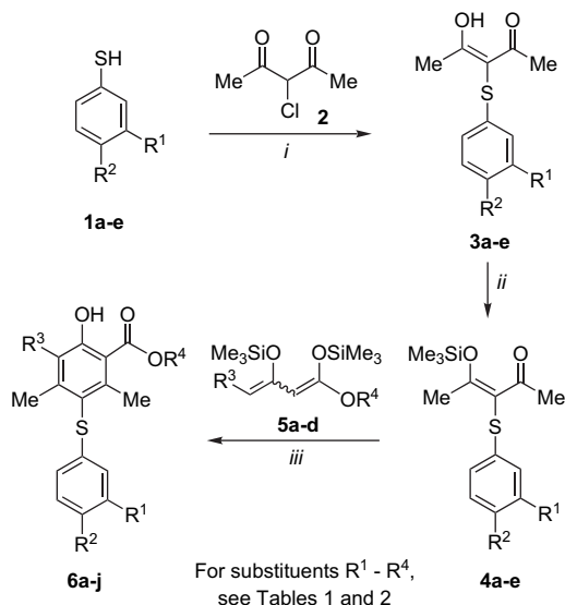
Scheme 1. Synthesis of 6a–j . Reagents and conditions: (i) method A: pyridine, MeOH, 0 \rightarrow 20 ^{\circ}\text{C} , 6 h; method B: piperidine, \text{CH}_2\text{Cl}_2 , MeOH, 0 \rightarrow 20 ^{\circ}\text{C} , 6 h; (ii) \text{Me}_3\text{SiCl} , \text{NEt}_3 , \text{C}_6\text{H}_6 , 20 ^{\circ}\text{C} , 72 h; (iii) \text{TiCl}_4 , \text{CH}_2\text{Cl}_2 , -78 \rightarrow 20 ^{\circ}\text{C} , 20 h.
