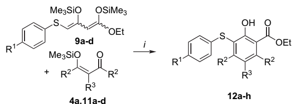
Scheme 3. Synthesis of 12a–h . Reagents and conditions: (i) \text{TiCl}_4 , \text{CH}_2\text{Cl}_2 , -78 \rightarrow 20^\circ\text{C} , 20 h.
