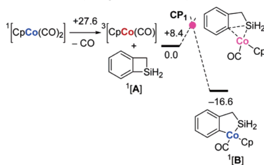
Scheme 5. Computed Pathway for the Formation of 1-Cobalta-2-silacyclopentene B at the DFT/B3LYP Level (energies in kcal/mol)
