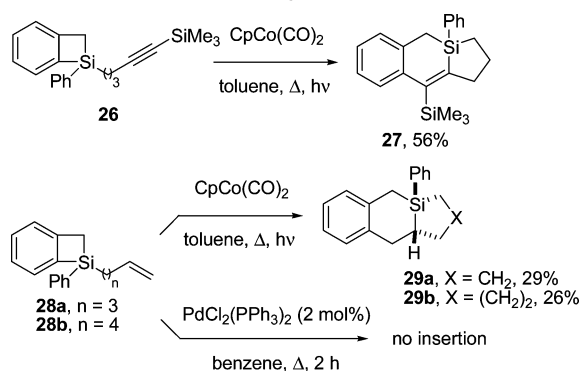
Scheme 4. One-Pot Intramolecular Cycloadditions of Three-Carbon Alkene- and Alkyne-Tethered Benzosilacyclobutenes
