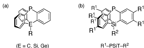
Figure 1. Structures of (a) phosphatriptycenes with a group 14 element on the other bridgehead and (b) 9-phospha-10-silatriptycenes with substituents \text{R}^1 and \text{R}^2 .
