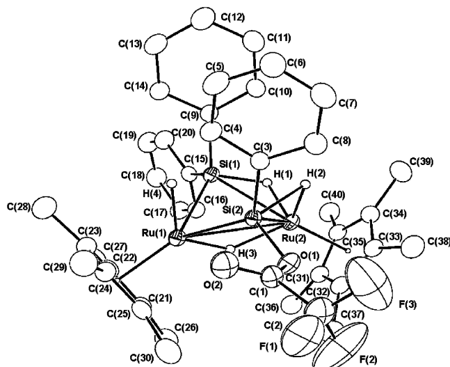
Figure 1. Molecular structure of (\text{Cp}^*\text{Ru})_2(\mu\text{-}\eta^2\text{-HSiPh}_2)\{\mu\text{-}\eta^2\text{-HSiPh}(\text{OCOCF}_3)\}(\mu\text{-H})(\text{H}) ( 2c ) with thermal ellipsoids at the 30% probability level. Hydrogen atoms except for those attached to the ruthenium atoms were omitted for clarity.
