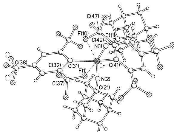
Fig. 1. Molecular structure of [\text{Cr}(\text{NAd})_2(\text{fmes})_2] ( 1 ), showing the disorder of one \text{CF}_3 group. H atoms are omitted for clarity.
