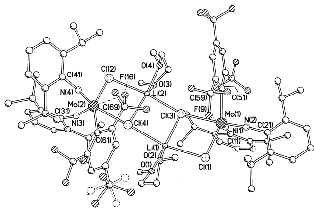
Fig. 3. Molecular structure of [\text{Mo}(\text{NC}_6\text{H}_3'\text{Pr}_2\text{-2,6})_2(\text{fmes})\text{Cl}]\cdot\text{LiCl}\cdot(\text{dme})_2 ( 3 ), showing the disorder of one \text{CF}_3 group. H atoms are omitted for clarity.
