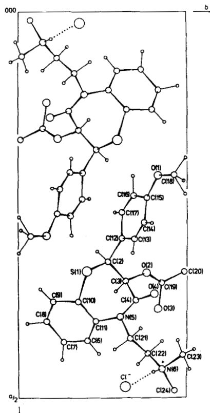
Fig. 4. Atom numbering, and molecular packing of (+)-1 showing N(6) \cdots Cl contact
