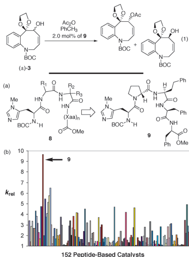
Figure 1. (a) Library of 152 catalysts for kinetic resolutions of 3 and the optimum member of the library, 9 . (b) Distribution of s -factors for library ( 8 ) observed for screening of substrate 3 (reactions conducted at 25 °C).
