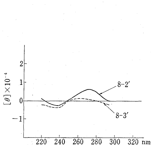
Fig. 4. CD Spectra of O-Cyclonebularines
