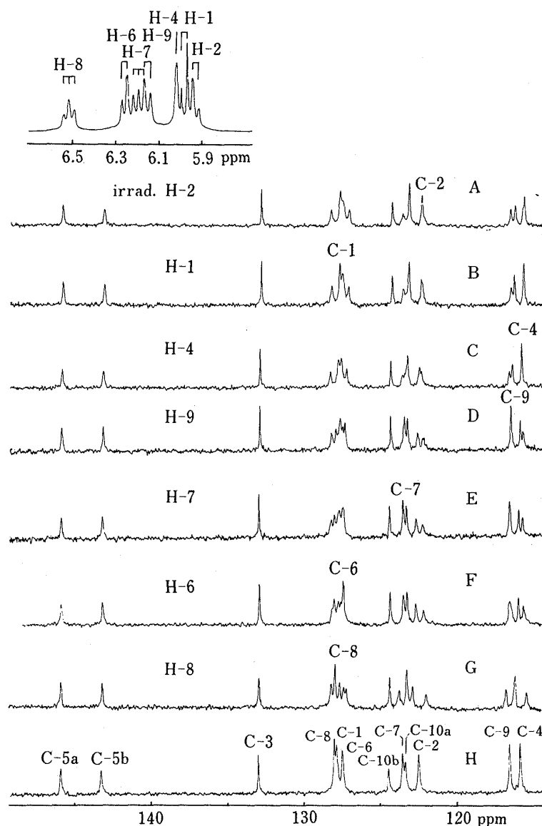
Fig. 3. ^1\text{H} - and ^{13}\text{C} -NMR Spectra of the Aromatic Region of CPZ in Aqueous Solution (33.3 mg/ml)
