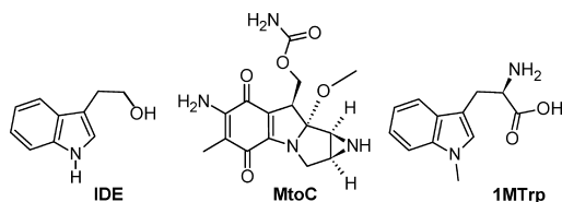
Scheme 1. Molecular Structures of 3-Indole Ethanol (IDE), Mitomycin C (MtoC), and 1-Methyl-tryptophan (1MTrp)
