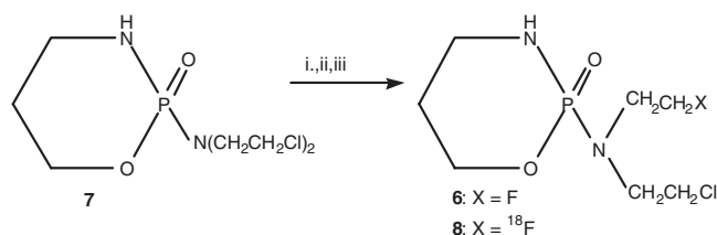
Figure 2. Direct halogen exchange synthesis of 6 and radiochemical synthesis of 2-[(2-chloro-2- ^{18}\text{F} fluoroethyl)amino]-2H-1,3,2-oxazaphosphorinane-2-oxide ( 8 ): (i) KF or ^{18}\text{F}^-/\text{K}_2\text{CO}_3/\text{acetonitrile} ; (ii) Kryptofix ® 222 110°C/10 min; (iii) chromatography
