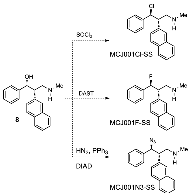
Scheme 9. Conversion of 7 to 9 and PCR200-SS
