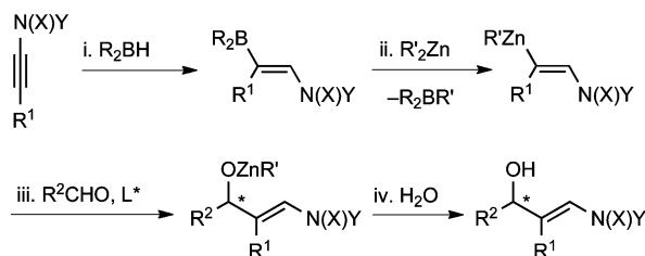
Scheme 2. One-Pot Generation of ( E )-Trisubstituted \beta -Hydroxy Enamines
