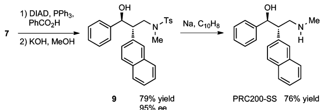
Scheme 9. Conversion of 7 to 9 and PCR200-SS
