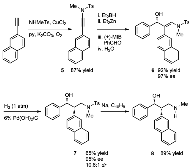
Scheme 7. Synthesis of the Key Intermediate 8 in the Synthesis of PRC200-SS and Derivatives
