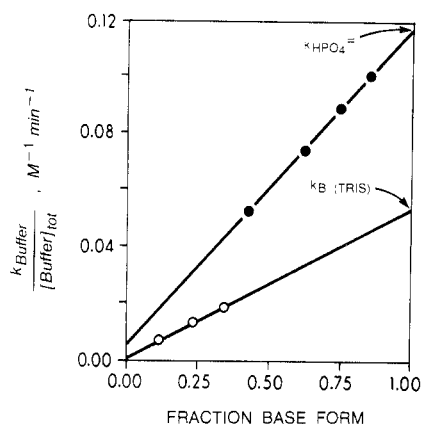
Figure 3. Effect of pH on buffer catalysis for the disappearance of 5 , 30 °C, \mu = 1.0 : (○) Tris buffer (1.0 M), k_B = 0.052 \text{ min}^{-1} ; (●) phosphate buffer (0.1 M), k_{\text{HPO}_4^{2-}} = 0.115 \text{ min}^{-1} . Lines represent best fit straight line determined by linear regression ( r^2 > 0.995 ).
