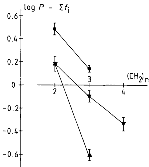
Fig. 3. The differences between experimental and calculated ( \Sigma f_i [31]) ( \log P )-values of aminoalkylbenz-amides vs. the length of the side-chain (—●—, compounds IIb and IIIb; —▲—, compounds IIc and IIIc; —▼—, compounds IIa-IVa)
