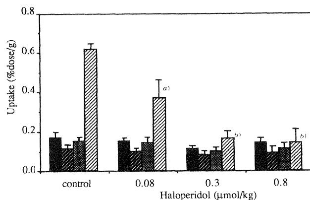
Fig. 1. Inhibition of [ ^{18}\text{F} ]4 Accumulation in Blood (■), Cerebellum (▨), Cortex (▩), and Striatum (▧) 90 min after i.v. Injection
