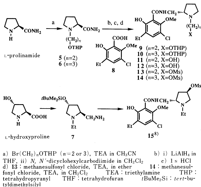
Chart 1. Syntheses of the Mesylate Precursors 13 , 14 , and 15
