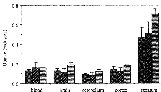
Fig. 2. Comparison of Tissue Distribution of [ ^{18}\text{F} ]4 90 min after i.v. Injection of Three Different Saline Solutions Containing Ethanol (■ EtOH), Hydrochloric Acid (▩ HCl), or Dimethylsulfoxide (▧ DMSO)
