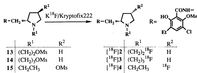
Chart 2. Radiochemical Syntheses of [\text{F}^{18}]\text{2} , [\text{F}^{18}]\text{3} , and [\text{F}^{18}]\text{4}
