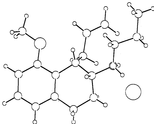
Figure 2. The X-ray crystallographic structure of 12a, confirmed as cis -( \pm )-1,2,3,4-tetrahydro-8-methoxy-1-(2-propenyl)- N - n -propyl-2-naphthalenamine hydrochloride.
