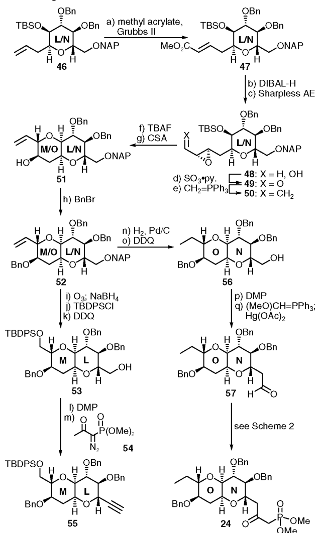
Scheme 5. Completion of the Furan-Based Synthesis of LM and NO Building Blocks 55 and 57 a
