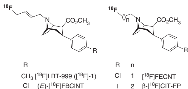
Figure 1 Chemical structures of [ ^{18}\text{F} ]LBT-999 and previously reported [ ^{18}\text{F} ]fluorinated tropane-analogues.
