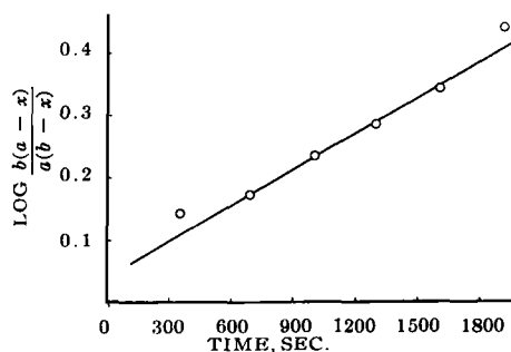
Fig. 5.—Typical bimolecular rate plot for the alkaline hydrolysis of atropine benzylchloride at 15.0°C. when alkali ( a ) and ester ( b ) are not equal.
