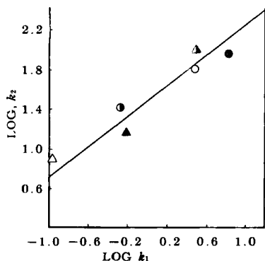
Fig. 8.—Plot showing the relationship of k_1 and k_2 of Reaction 1 and Reaction 2 for the following compounds at 30°C.: \Delta , tropine phenylacetate; \blacktriangle , atropine; \bullet , nor-atropine; \circ , tropine p -nitrobenzoate; \triangle , homatropine; \bullet , tropine phenoxyacetate.
