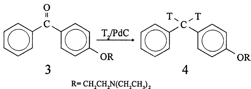
Figure 2. Synthesis of [ ^3\text{H} ]DPPE ( 4 ) from DBPE ( 3 ).
