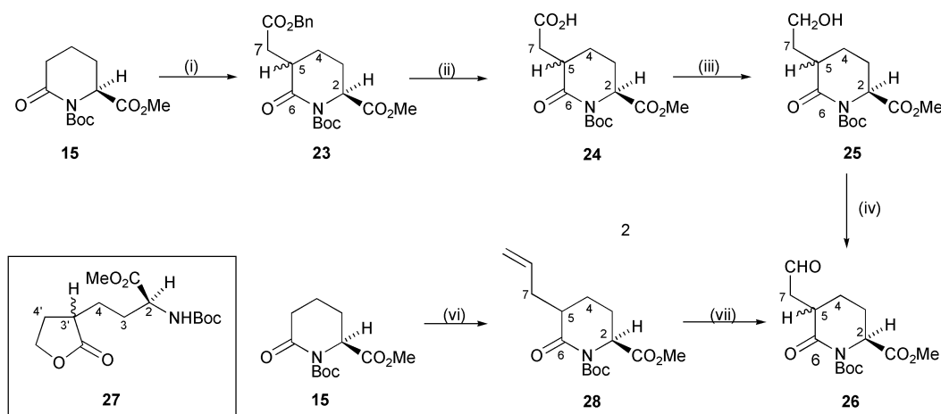
Scheme 3 (i) LHMDS–BrCH 2 CO 2 Bn (56%); (ii) H 2 –Pd–C (88%); (iii) H 3 B·SMe 2 (55%) (iv) ClCOCOCl–DMSO (20%); (vi) LHMDS–allylBr–THF (45%); (vii) O 3 –Ph 3 P (72%).
