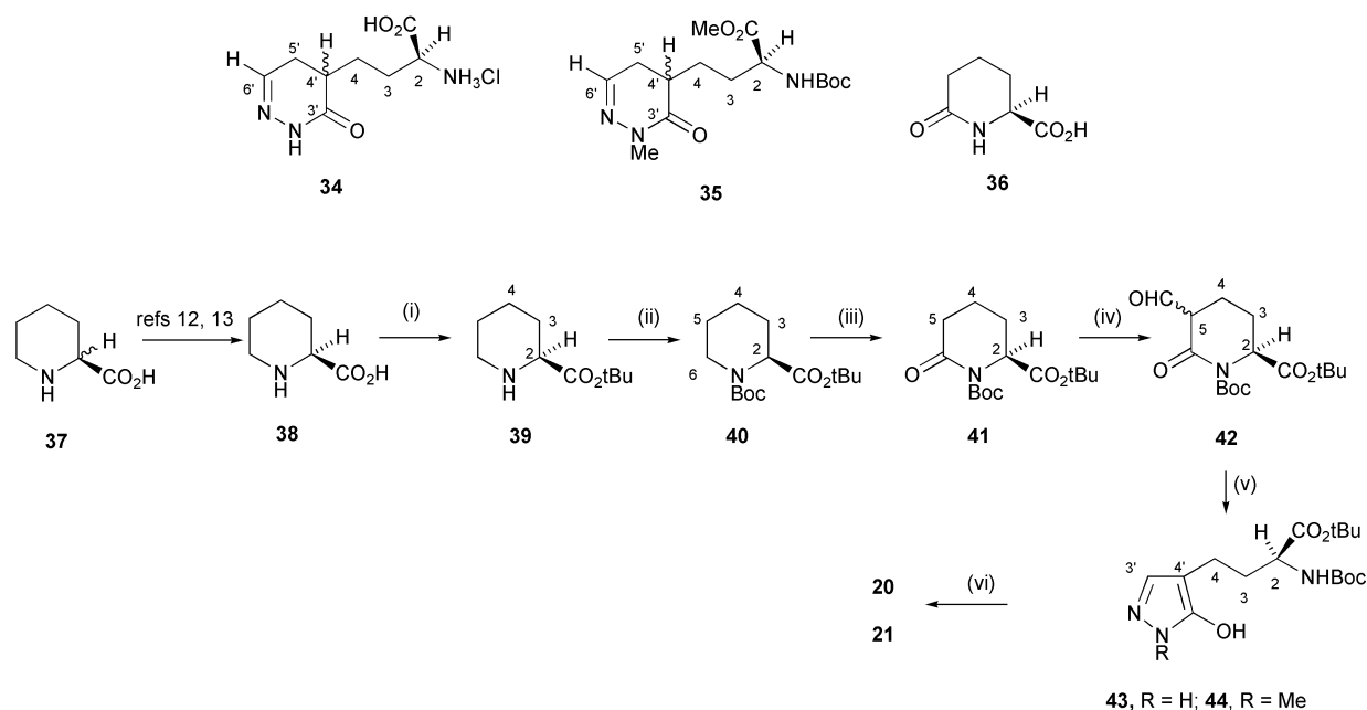
Scheme 5 (i) t\text{BuOAc-HClO}_4 (54%); (ii) \text{Boc}_2\text{O-NaHCO}_3 (85%); (iii) (a) \text{RuCl}_3\cdot\text{H}_2\text{O} (b) \text{NaIO}_4\text{-EtOAc-H}_2\text{O} (83%), (ee >99%); (iv) LHMDS- \text{HCO}_2\text{Me} ; (v) \text{RNHNH}_2\text{-MeOH} [43 46%, 44 42% for (iv) + (v)]; (vi) 6 N aq. \text{HCl} (20, 89%, 21 91%).
