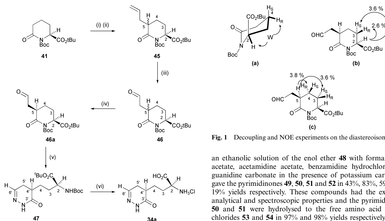
Scheme 6 (i) LHMDS-allylBr (59%, 1:1 cis:trans ); (ii) (a) LHMDS, (b) 2, 6-di- tert -butylphenol (84% 9:1 cis:trans ); (iii) (a) \text{O}_3\text{-CH}_2\text{Cl}_2 -78 °C, (b) \text{PPh}_3 (85%); (iv) separate; (v) \text{H}_2\text{NNH}_2\text{-MeOH} (88%); (vi) 6 N \text{HCl} (94%).
