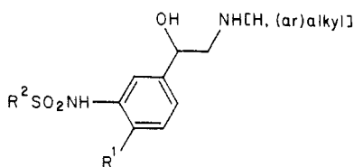
23a, R^1 = H; R^2 = (ar)alkyl b, R^1 = OH; R^2 = (ar)alkyl c, R^1 = OH; R^2 = \text{CH}_2\text{F}
