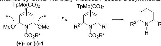
Scheme 2. Preparation of Pseudo-Symmetrical Dimethoxy Complex 1 a
